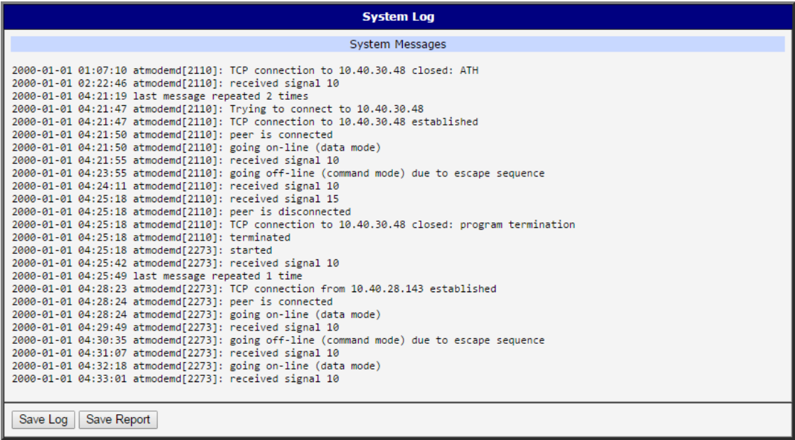
Figure 5: System Log
